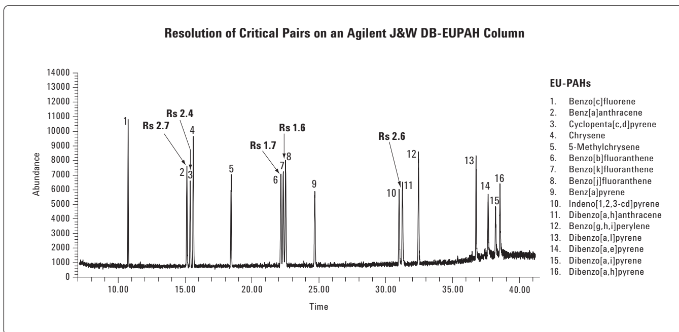
Figure 1. TIC of a 0.5 µL injection of 0.5 ng EU priority PAH standard solution on an Agilent J&W DB-EUPAH 20 m × 0.18 mm, 0.14 µm capillary GC column (Agilent p/n 121-9627). Chromatographic conditions are listed in Table 1.
